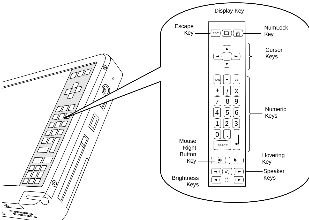
Figure 2-1 Stylistic Hotpad Arrays
