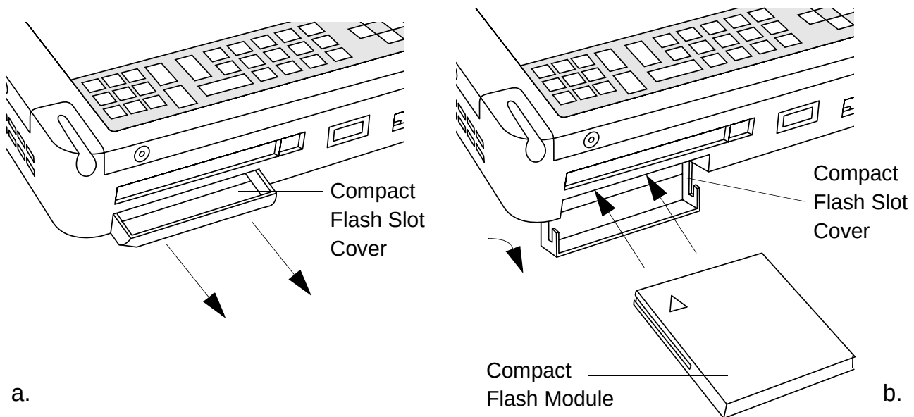
Figure 2-3 Installing a Compact Flash Module
