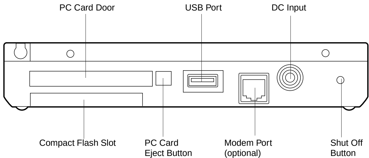
Figure 1-4 Right-Side Connectors and Interfaces
