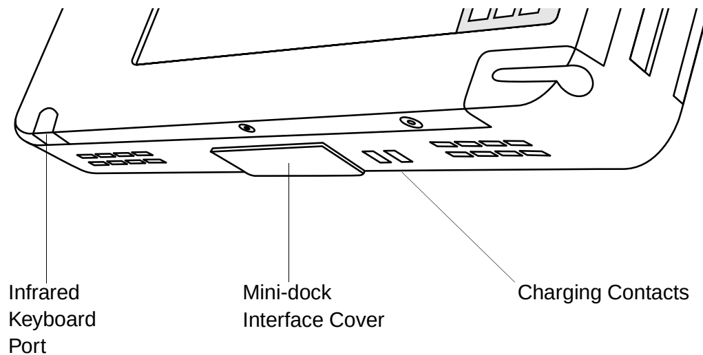
Figure 1-6 Bottom Connectors and Interfaces
