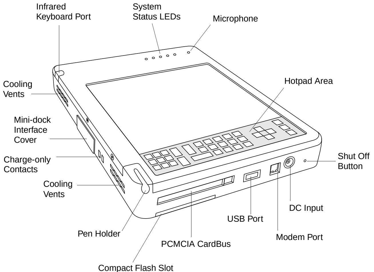
Figure 1-1 StylisticLT C-500 PenTablet Features (Front View)
