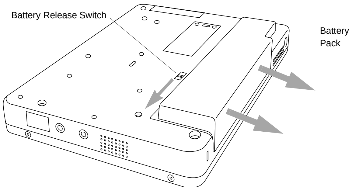
Figure 2-2 Removing the Battery Pack
