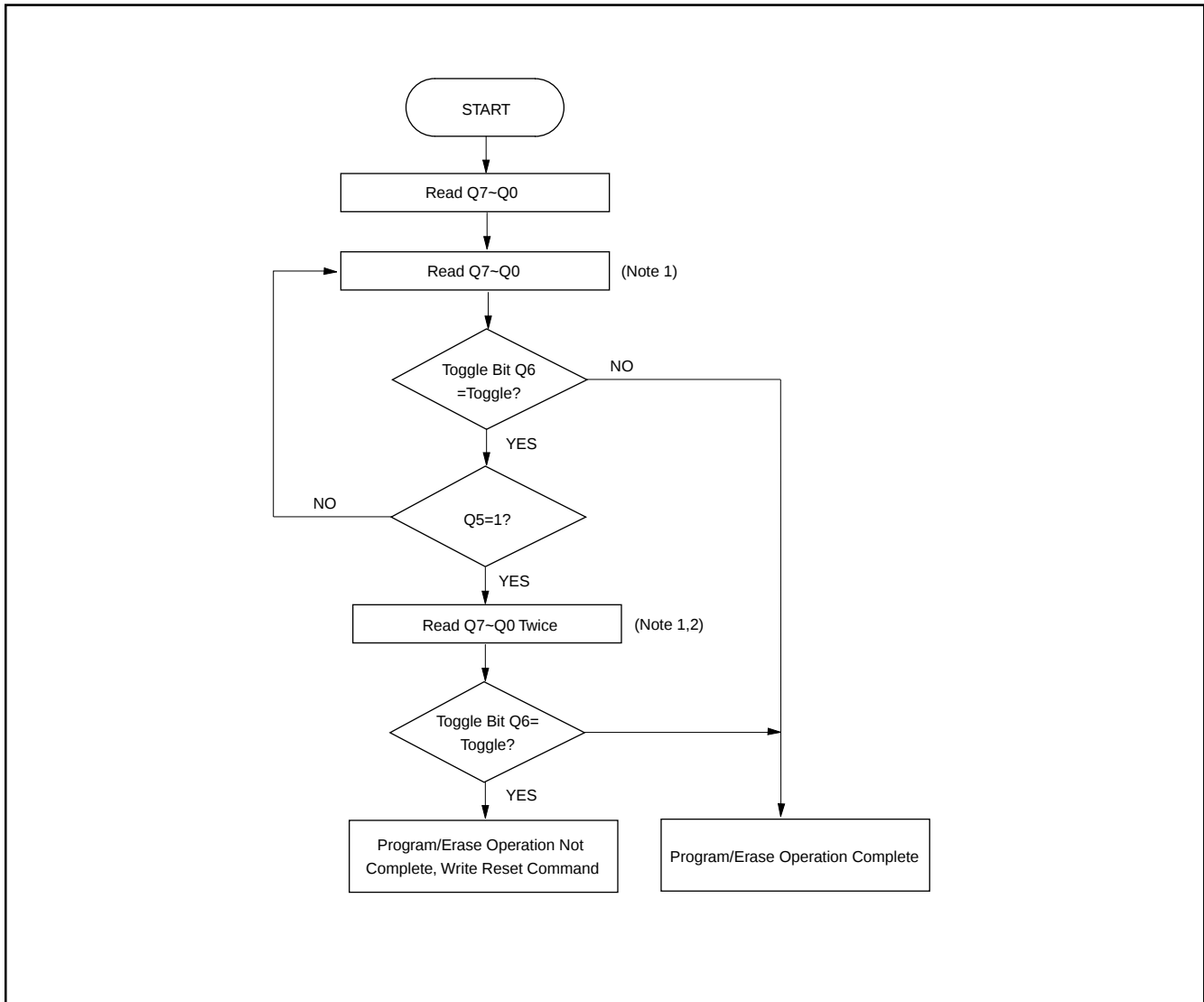
Fig 16. TOGGLE BIT ALGORITHM
