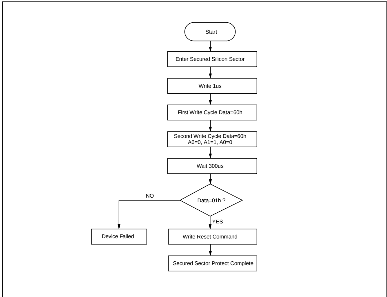
Fig 11. SECURED SILICON SECTOR PROTECTED ALGORITHMS FLOWCHART
