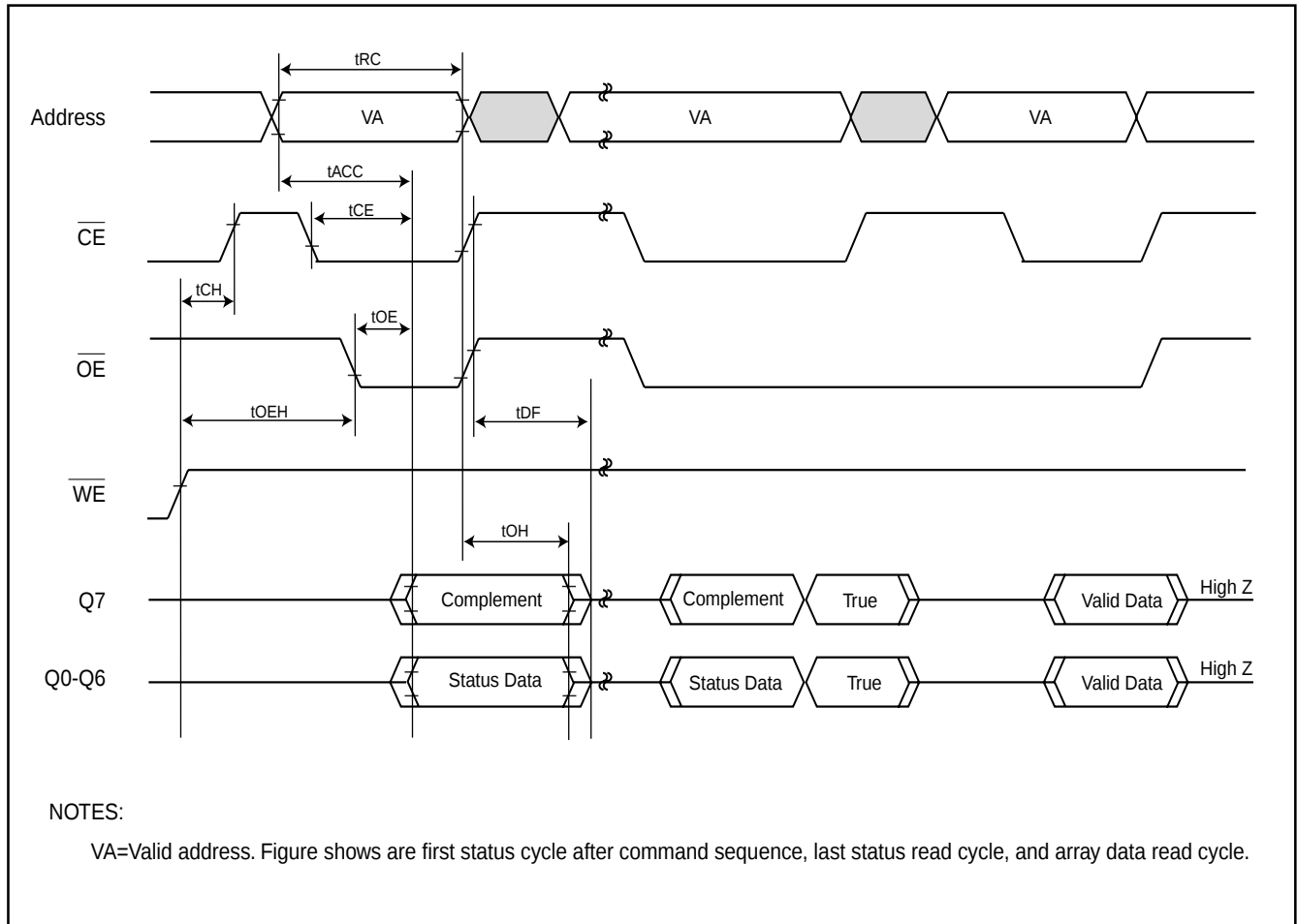
Fig 13. DATA POLLING TIMING WAVEFORMS (DURING AUTOMATIC ALGORITHMS)
