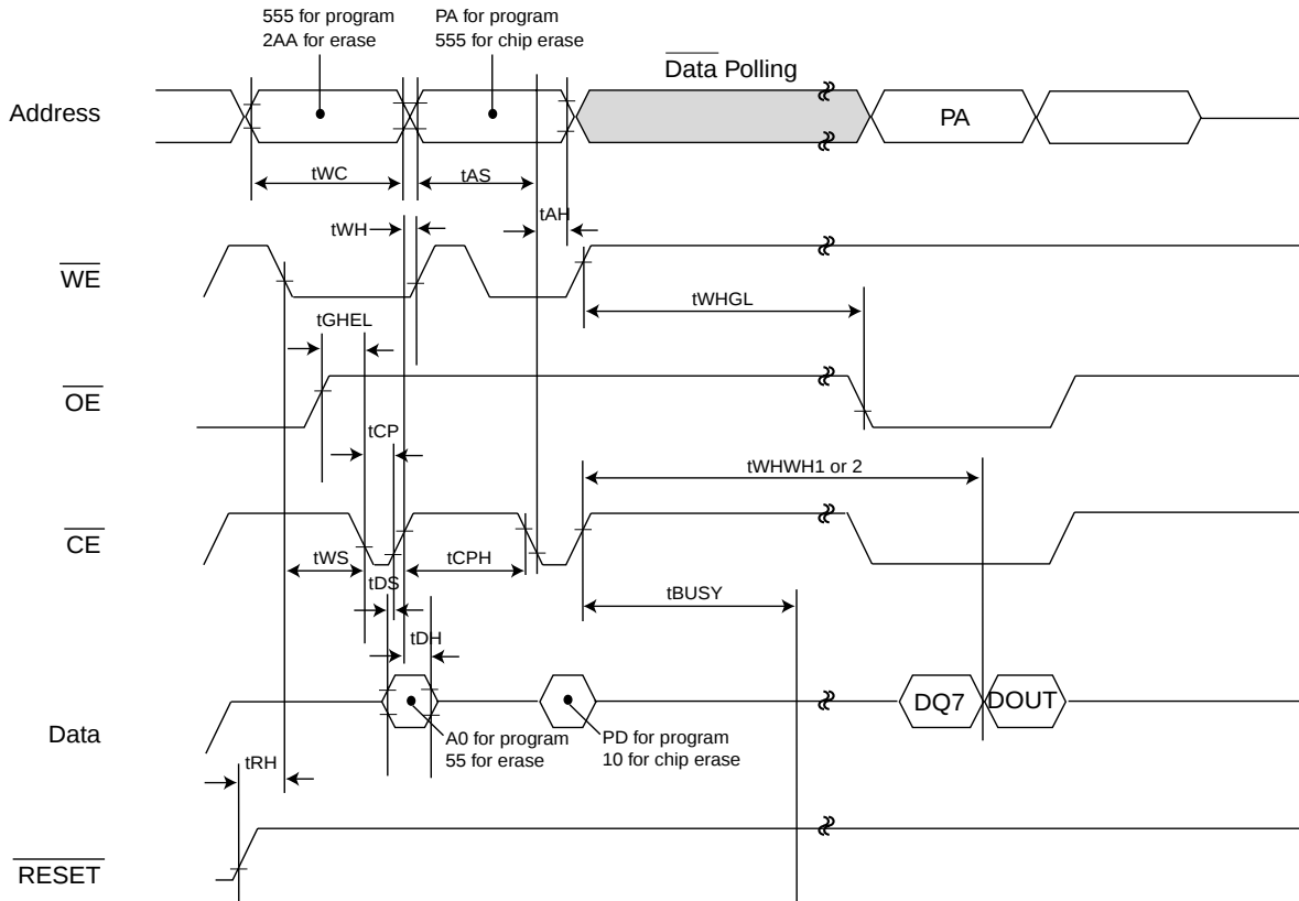
Fig 8. \overline{\text{CE}} CONTROLLED PROGRAM TIMING WAVEFORM
