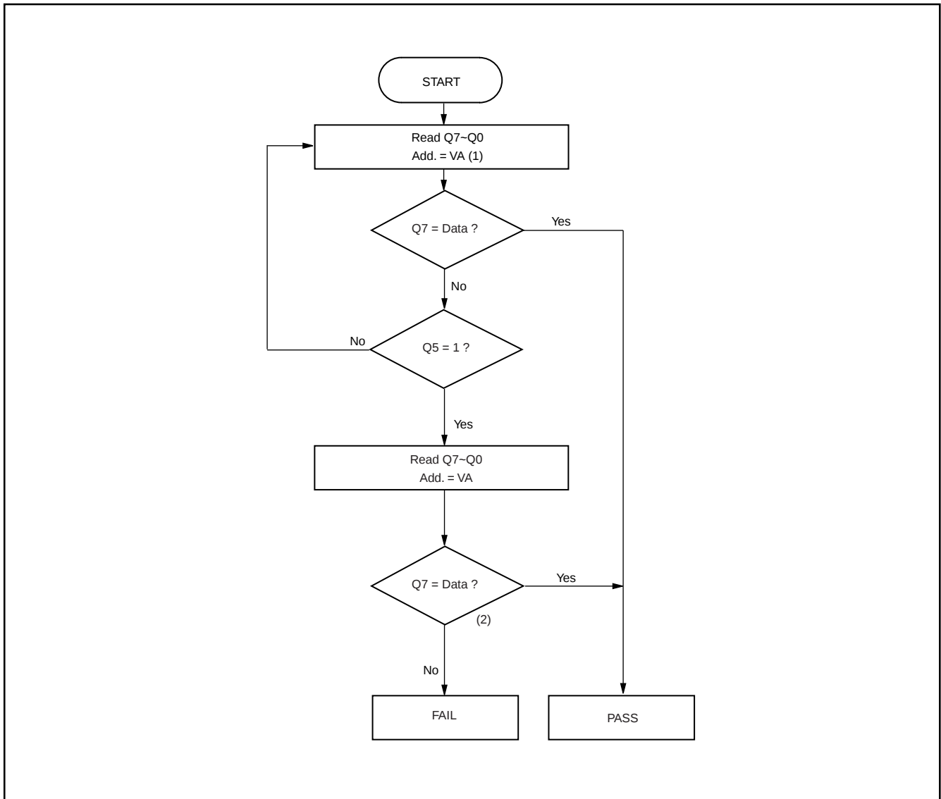
Fig 14. DATA POLLING ALGORITHM
