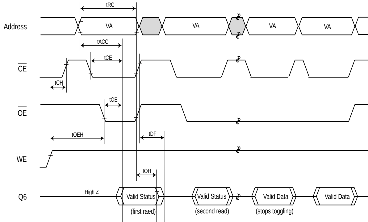
Fig 15. TOGGLE BIT TIMING WAVEFORMS (DURING AUTOMATIC ALGORITHMS)
