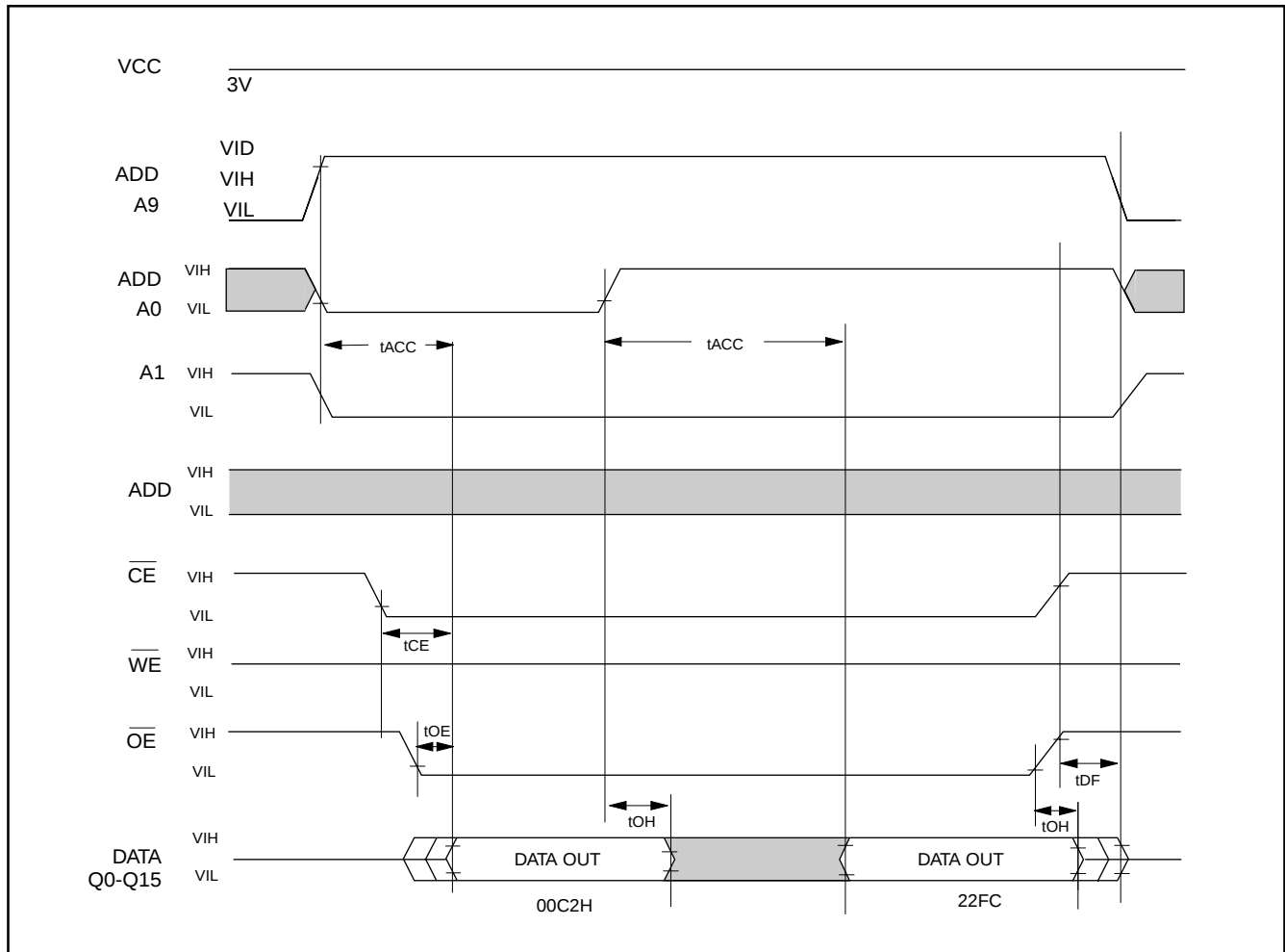
Fig 12. SILICON ID READ TIMING WAVEFORM
