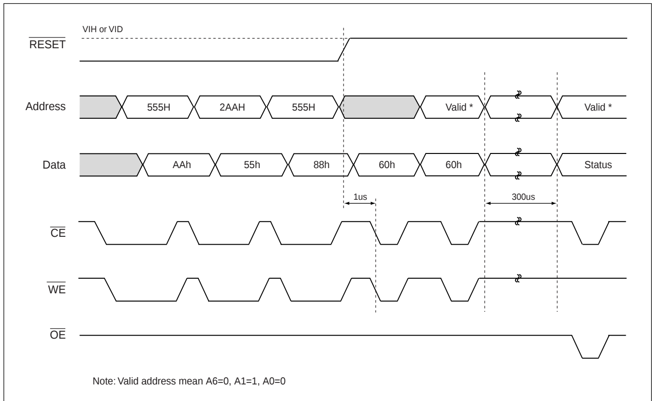
Fig 10. SECURED SILICON SECTOR PROTECTED TIMING WAVEFORM
